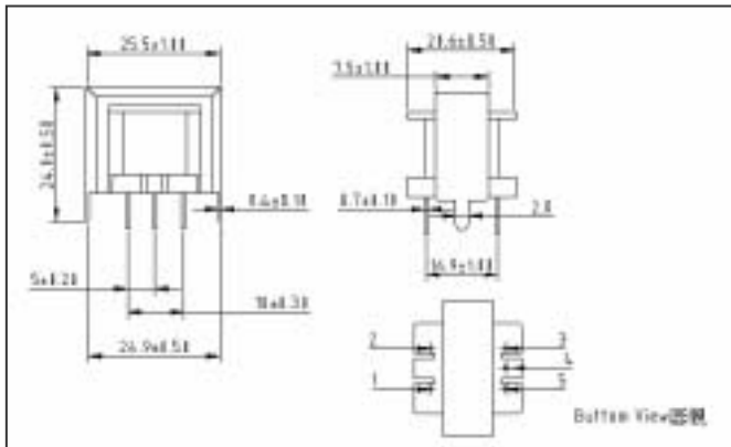
EE5 Transformer
